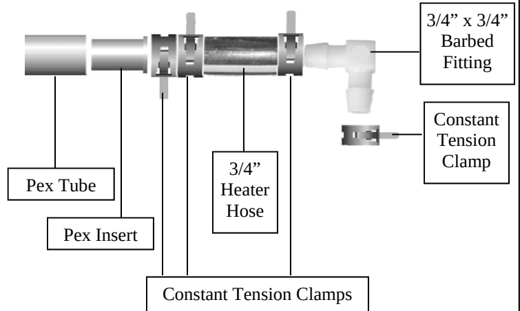
90° Connection Components
